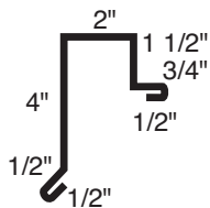
Maximum Vent Pan
