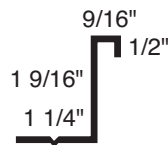
Mechanical Seam Clip SSR
