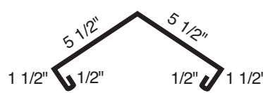
Hip & Ridge Cap SSR
