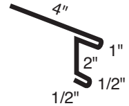
Eaves Trim SSR
