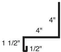
Skylight Flashing #1 SSR
