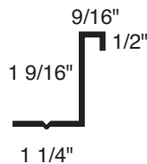
Mechanical Seam Clip
