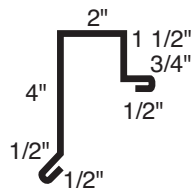
Maximum Vent Pan
