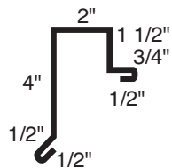
Turbine Pan
