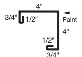
Outside Corner
