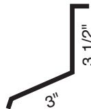
Under Bent Wall Flashing
