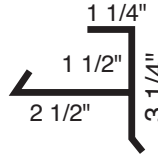
F-Gable Flashing
