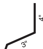
Snow / Ice Stop
