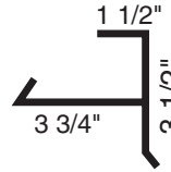
F-Gable Flashing
